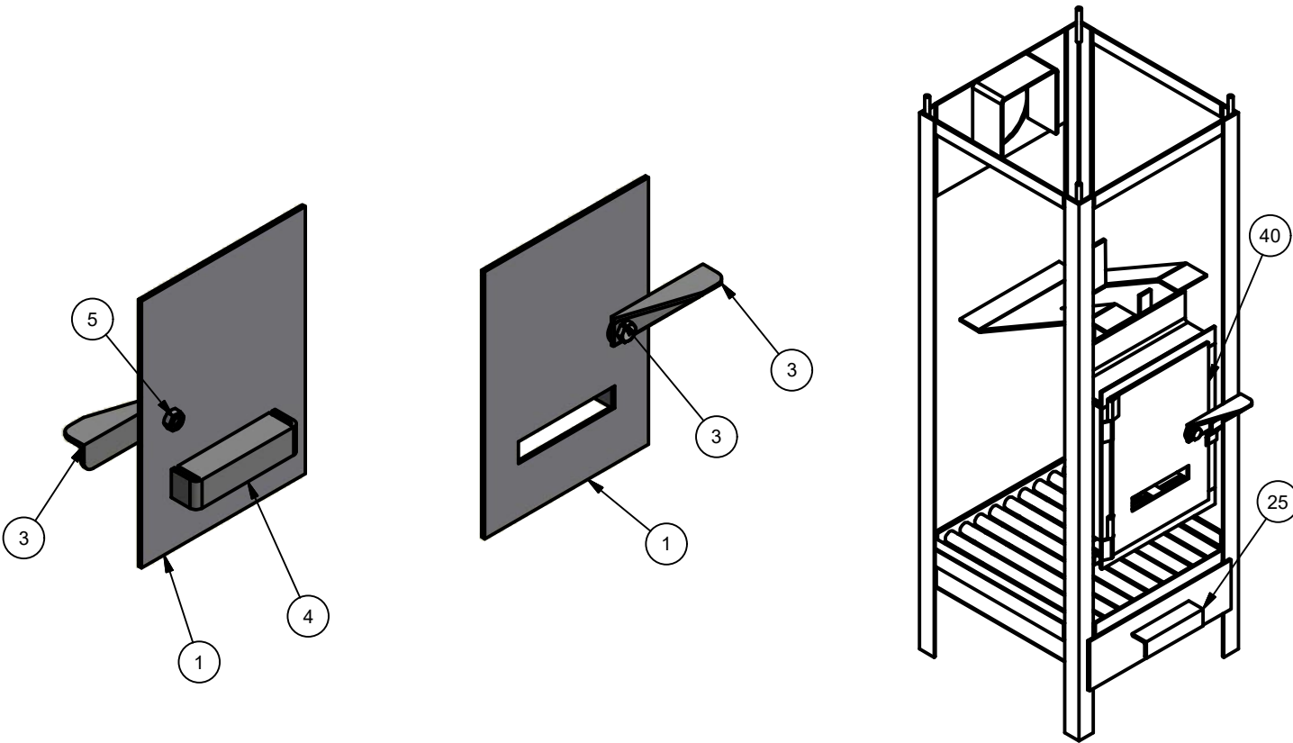
VISTA133 ( 1:8.5 )
