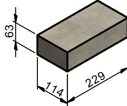
LADRILLO REFRACTARIO ( 1:10 )
