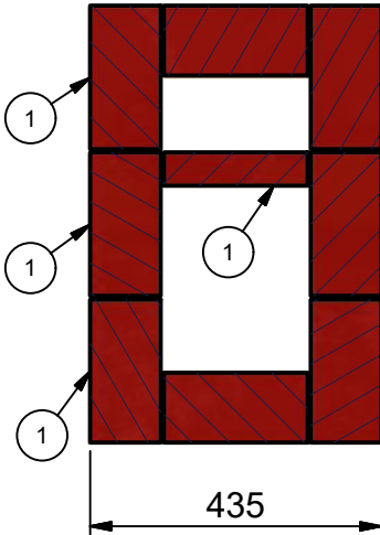
18-18 ( 1:12.5 )
