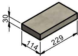
LADRILLO REFRACTARIO ( 1:10 )
