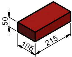
TEJUELA REFRACTARIA 3CM ( 1:10 )
