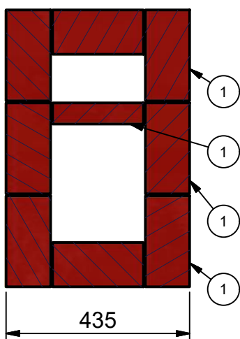
16-16 ( 1:12.5 )
