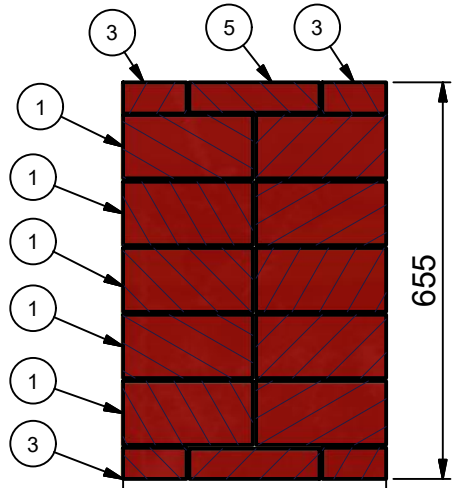
22-22 ( 1:12.5 )
